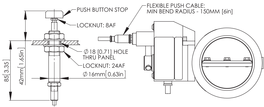
REMOTE PUSH BUTTON MANUAL STOP OPTION: ORDER CODE EXX
